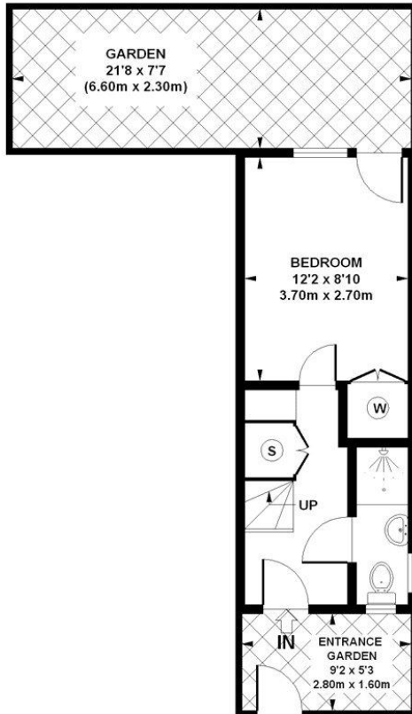
GROUND FLOOR GROSS INTERNAL FLOOR AREA 215 SQ FT
